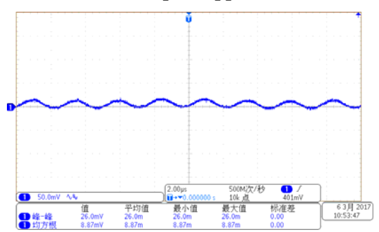
Output Ripple
